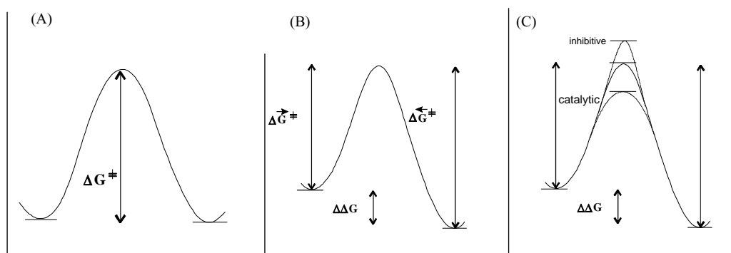
Fig. 6. Effect of stationary phase catalytic or inhibitive effect on the energy barrier and hence kinetics of interconversion of molecules A and B. (A) Process with similar ground state energies of the two molecules. (B) Situation where the forward and reverse reactions can have different energy and kinetics. (C) Possible effect of the stationary phase in altering the kinetics by increasing or decreasing the energy of the interconversion.
