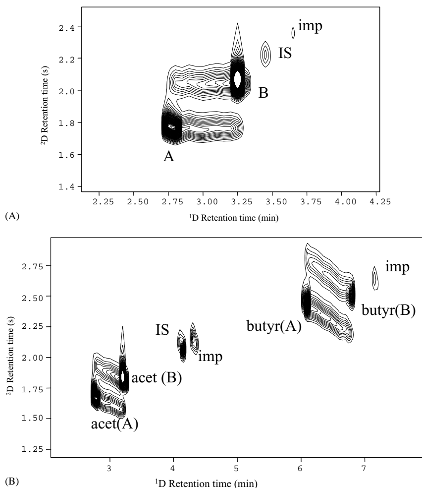
Fig. 4. Comparison of the effect of isothermal oven operation, against temperature programmed operation, for the comprehensive two-dimensional gas chromatography experiment in DGC × DGC. Column set [1, 6 (0.8)]. (A) Acetaldoxime with n -hexanol (IS) at 70 °C, 20 p.s.i., 3 s modulation. (B) Acetaldoxime and butyraldoxime with n -hexanol (IS) at 70 °C for 2.5 min heated to 100 °C at 5 °C/min, 20 p.s.i., 3 s modulation. imp: impurity in the starting materials.
