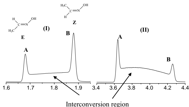
Fig. 2. The classic dynamic chromatogram has original injected peaks A and B, and an interconversion or plateau region arising from molecular structural change during chromatographic elution. (I) Acetaldoxime and (II) butyraldoxime, where the initial amount of A isomer is less for acetaldoxime (the E -isomer) and more for butyraldoxime.
