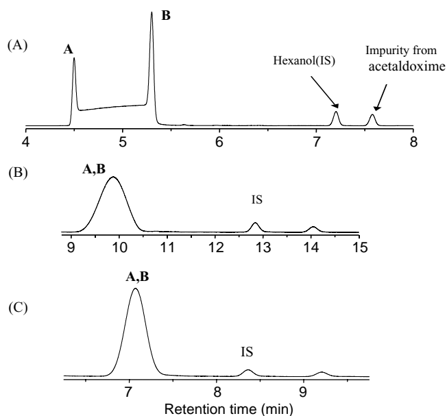
Fig. 3. As the rate or extent of interconversion increases, the two isomer peaks, which are originally well resolved (A, 70^\circ\text{C} ; 20 p.s.i.; 1 p.s.i. = 6894.76 Pa), progressively collapse into a single peak whose extremities are determined by the retention properties of the individual isomers (B, 90^\circ\text{C} ; 5 p.s.i.), and then into a much narrower peak which now will have width much more like a normal GC peak (C, 110^\circ\text{C} ; 5 p.s.i.). Note that since these conditions are brought about by increases in temperature or reduced flow rate, the relative peak retentions will change: they are shown here approximately normalised to the retention of the peak set.
