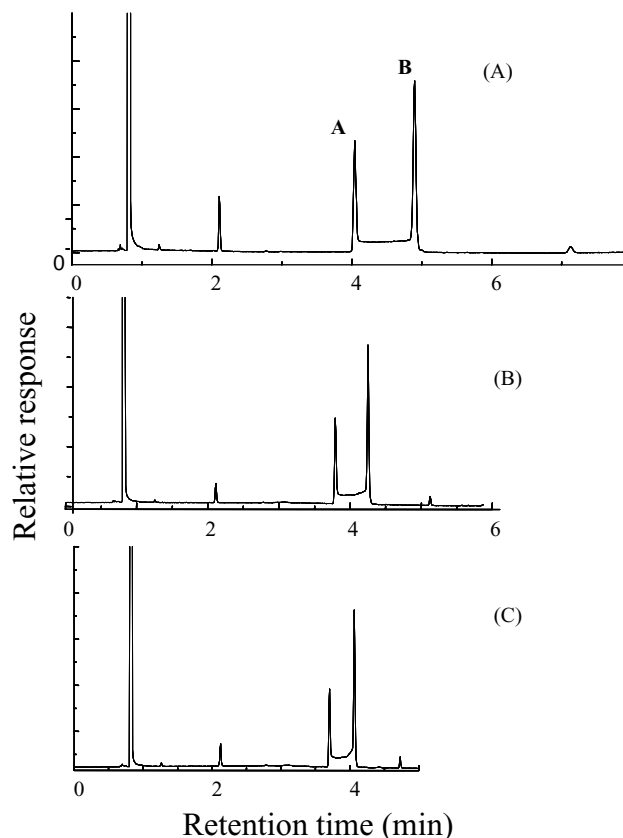
Fig. 5. Effect of temperature programming on the interconversion plateau for acetaldoxime (A) Isothermal 60 °C; (B) 60 °C for 3 min, followed by temperature programming at 15 °C/min; (C) 60 °C for 3 min, followed by temperature programming at 25 °C/min.
