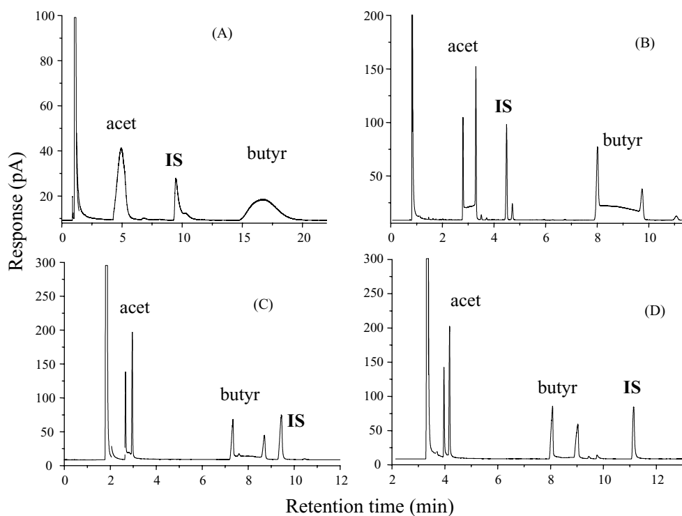
Fig. 7. Comparison of extents of interconversion on a selection of different stationary phases, under different experimental conditions of temperature and pressure. (A) BP20 at 40 °C, 25 p.s.i.; (B) BP21 at 70 °C, 20 p.s.i.; (C) BP10 at 60 °C, 15 p.s.i.; (D) BPX5 at 60 °C, 20 p.s.i.
