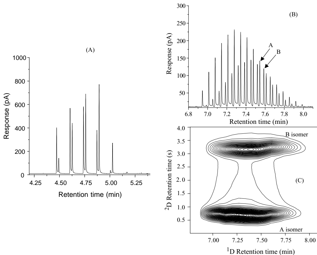
Fig. 9. Illustration of effect of fast interconversion, giving only one apparent peak on ^1D , and with interconversion on ^2D using column set [1, 6 (4.0 m)]. (A) Acetaldoxime; oven 90 °C, 8 s modulation. (B) Butyraldoxime; oven 100 °C, 4 s modulation.
