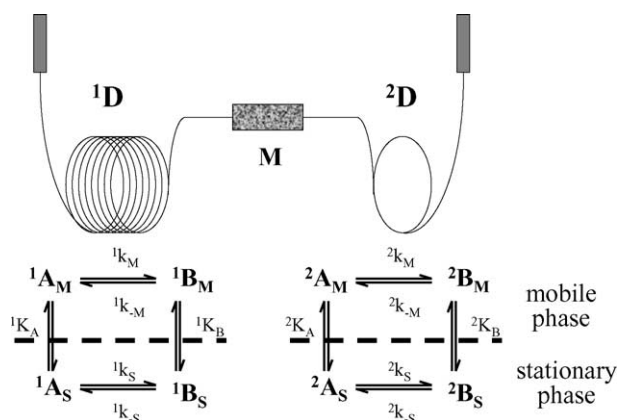
Fig. 1. Illustration of the dynamic interconversion system A \rightleftharpoons B for isomers A and B. K are chromatographic distribution constants; k is the interconversion rate constant for A \rightarrow B and k_{-} is for the reverse process; subscripts M and S refer to mobile phase and stationary phase, respectively. In a two-dimensional system, the first ( ^1D ) and second ( ^2D ) columns may be different phases, and so have different kinetic parameters indicated by superscript ^1 and ^2 , respectively. The cryogenic modulator M provides the mechanism for modulating the first dimension peak to the second column.
