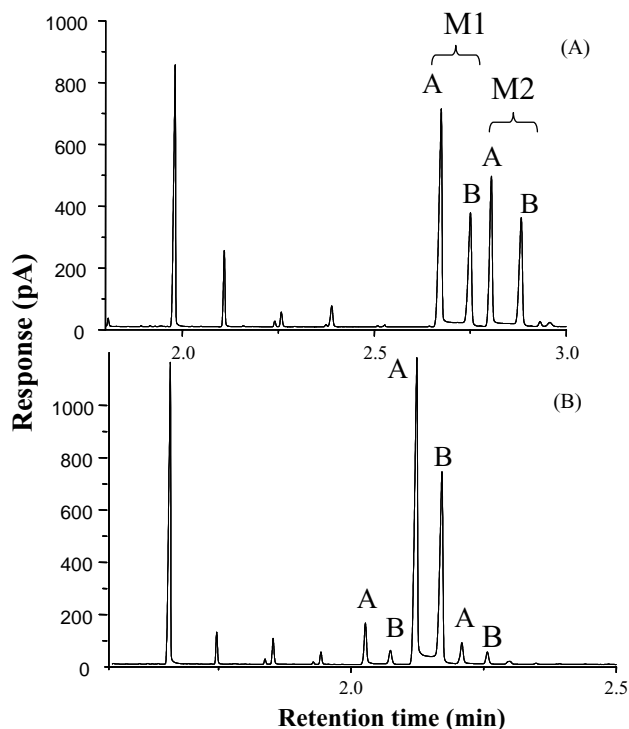
Fig. 8. Interconversion of butyraldoxime on the ^2D column using column set [2, 6 (4.0)] under differing temperature conditions. (A) 80 °C; 8.0 s modulation; (B) 90 °C, 5.5 s modulation. A and B denote the two isomers, and M1 and M2 denote two successive modulation events over the first column peak elution. For (B), three modulations can be seen. Since there are few modulations, it is apparent that the peak elution from the first column is both rather narrow, and that also there is fast interconversion on this column.
